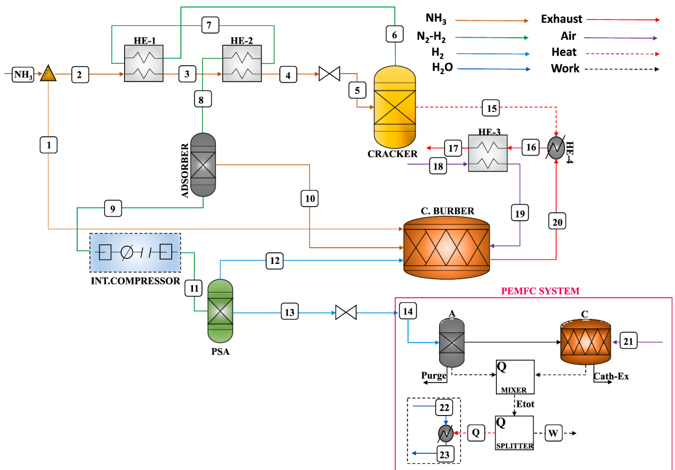
Fig. 3. Layout of NH 3 -based PEMFC power generation system.
