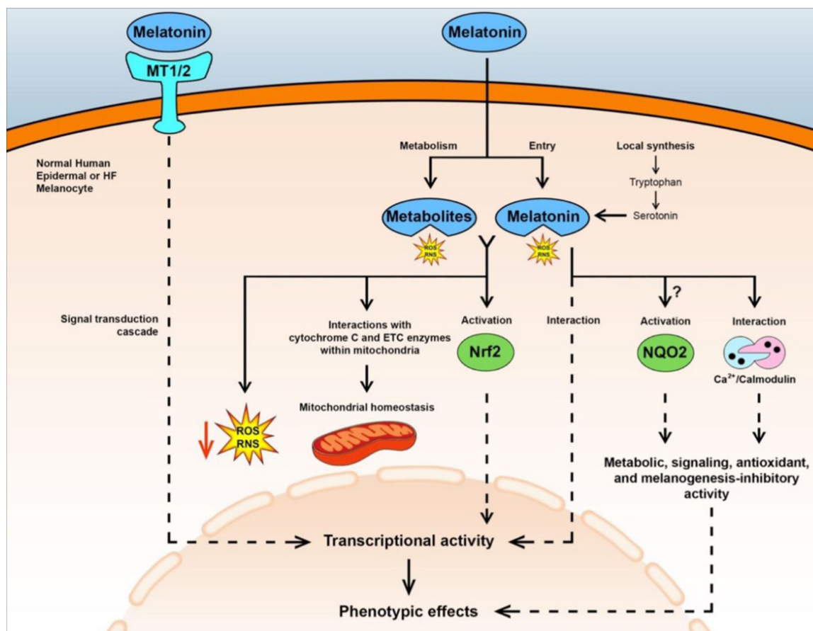
FIGURE 1 Schematic summary of melatonin's effects in human epidermal and HF melanocytes. Exogenous or endogenously synthesized melatonin can regulate phenotype in these cells through interactions with membrane-bound MT1/2 receptors NQO2, and the calcium/calmodulin complex or through stimulation of Nrf2 (reviewed in Slominski et al. 86 ). However, it is not fully understood if melatonin activates NQO2, a detoxifying enzyme. 7,87,88 Noteworthy phenotypic effects of melatonin include melanogenesis inhibition, and stimulation of DNA repair, and expression and activity of antioxidant enzymes (e.g., superoxide dismutase and catalase) (reviewed in Slominski et al. 8 ). Melatonin may also be transported to different subcellular compartments, but the detailed mechanism is not fully understood. 63 Furthermore, melatonin can be synthesized within these melanocytes. Melatonin and its metabolites, such as cyclic-3-hydroxymelatonin (C-3HOM) and N-acetyl-5-methoxykynuramine (AMK), directly scavenge ROS/RNS 89,90 and help maintain mitochondrial homeostasis through interactions with cytochrome C and enzymes of the ETC. Specifically, cytochrome C within mitochondria is thought to be involved in the conversion of melatonin to its potent antioxidant metabolite, N(1)-acetyl-N(2)-formyl-5-methoxykynuramine (AFMK), 91 and its secondary product, AMK, when in the presence of hydrogen peroxide. 92 Also, melatonin may interact with cytochrome C and ETC enzymes within mitochondria to promote mitochondrial homeostasis and decrease free radical formation. 93 Furthermore, melatonin may affect the transcription of peripheral clock genes Bmal1 and Per1 with alterations in melanogenesis and other melanocyte activities. 65,94,95 Direct effects are shown by solid lines and multiple reactions and signaling are shown by dashed lines. ETC, electron transport chain; HF, hair follicle; MT1/2, melatonin receptors 1 and 2; NQO2, N-ribosyldihydronicotinamide:quinone reductase 2; Nrf2, nuclear factor erythroid 2-related factor 2; RNS, reactive nitrogen species; ROS, reactive oxygen species
