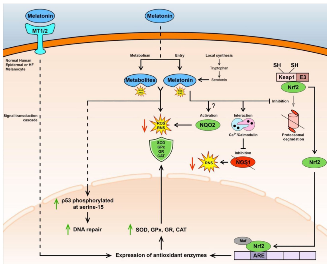
FIGURE 3 Schematic summary describing antioxidant defense mechanisms by melatonin and its metabolites in human melanocytes. Melatonin can bind to MT1 and MT2 receptors on the cell membrane, triggering a signaling cascade that leads to the expression of antioxidant enzymes (e.g., SOD, GPx, GR, and CAT) for defense against ROS and RNS. 89,189 Melatonin may also be transported to the cytoplasm, but the detailed mechanism is not fully understood. 63 Furthermore, melatonin can be synthesized within these melanocytes. Melatonin and its metabolites, such as C-3HOM and AMK, can directly scavenge ROS/RNS. 89,90 Furthermore, melatonin and its metabolites, including AFMK, 6-OHM, 5-MT, and NAS, protect human epidermal melanocytes from UV-B-induced damage/apoptosis by enhancing phosphorylation of p53 at Serine 15, thereby leading to activated p53 accumulation in the nucleus and stimulation of DNA repair. 28 Melatonin may activate NQO2, thereby reducing oxidative stress, 190,191 however, this mechanism's presence in these melanocytes is not fully understood. 7 Melatonin at concentrations higher than 1 nM within the cell can interact with the calcium/calmodulin complex leading to inhibition of NOS1-mediated generation of RNS, with potential reductions in RNS levels. 63 Melatonin may also inhibit the Keap1-E3 ligase complex and the ubiquitination and proteasomal degradation of Nrf2, thereby preserving high Nrf2 levels that translocate to the nucleus. In the nucleus, Nrf2 may couple with Maf, a transcription factor, allowing Nrf2 to bind ARE on the promoter region of genes encoding antioxidant enzymes (e.g., SOD and GPx), resulting in their increased expression and activity, which then convert ROS and RNS to unreactive products. 1 Direct effects are shown by solid lines and multiple reactions and signaling are shown by dashed lines. CAT, catalase; GPx, glutathione peroxidase; GR, glutathione reductase; RNS, reactive nitrogen species; ROS, reactive oxygen species; SOD, superoxide dismutase
