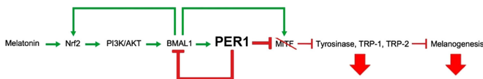
FIGURE 4 Schematic summary describing hypothesized mechanisms by which melatonin may regulate melanogenesis in normal human epidermal and HF melanocytes. Melatonin may activate the PI3K/AKT pathway, via Nrf2 activation, 28 to stimulate expression of Bmal1 , thereby increasing BMAL1 levels. 95 BMAL1 may increase expression of Nrf2 to further stimulate this PI3K/AKT pathway 240 and PER1 to inhibit MITF downstream. 186 PER1 also translocates to the nucleus and inhibits transcriptional activity of BMAL1, 241,242 thereby preventing BMAL1's stimulation of MITF transcription. 243 Decreased MITF levels lead to decreased expression of melanogenesis enzymes tyrosinase, TRP-1, and TRP-2 and results in decreased melanogenesis. 94
